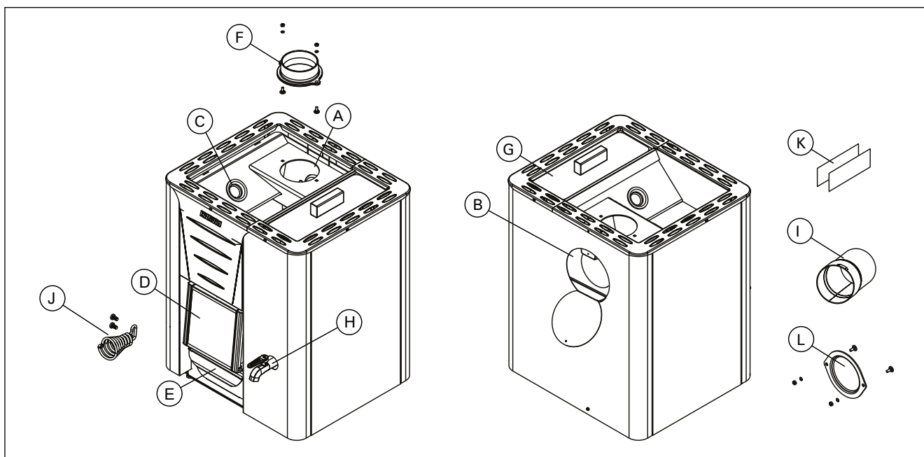
Figure 1. Stove parts. Unauthorised modification of the stove is prohibited.
